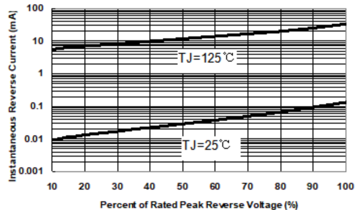
Fig.2-Typical Reverse Characteristics
